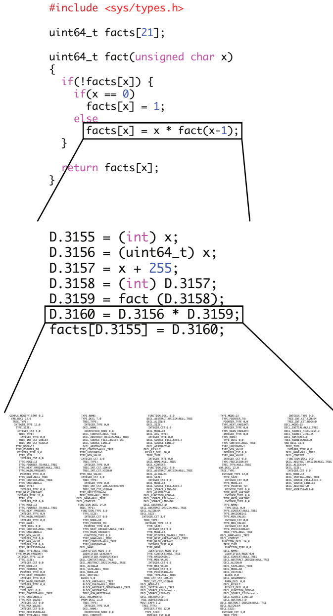
Figure 1: An example showing the C to intermediate representation blow-up.
