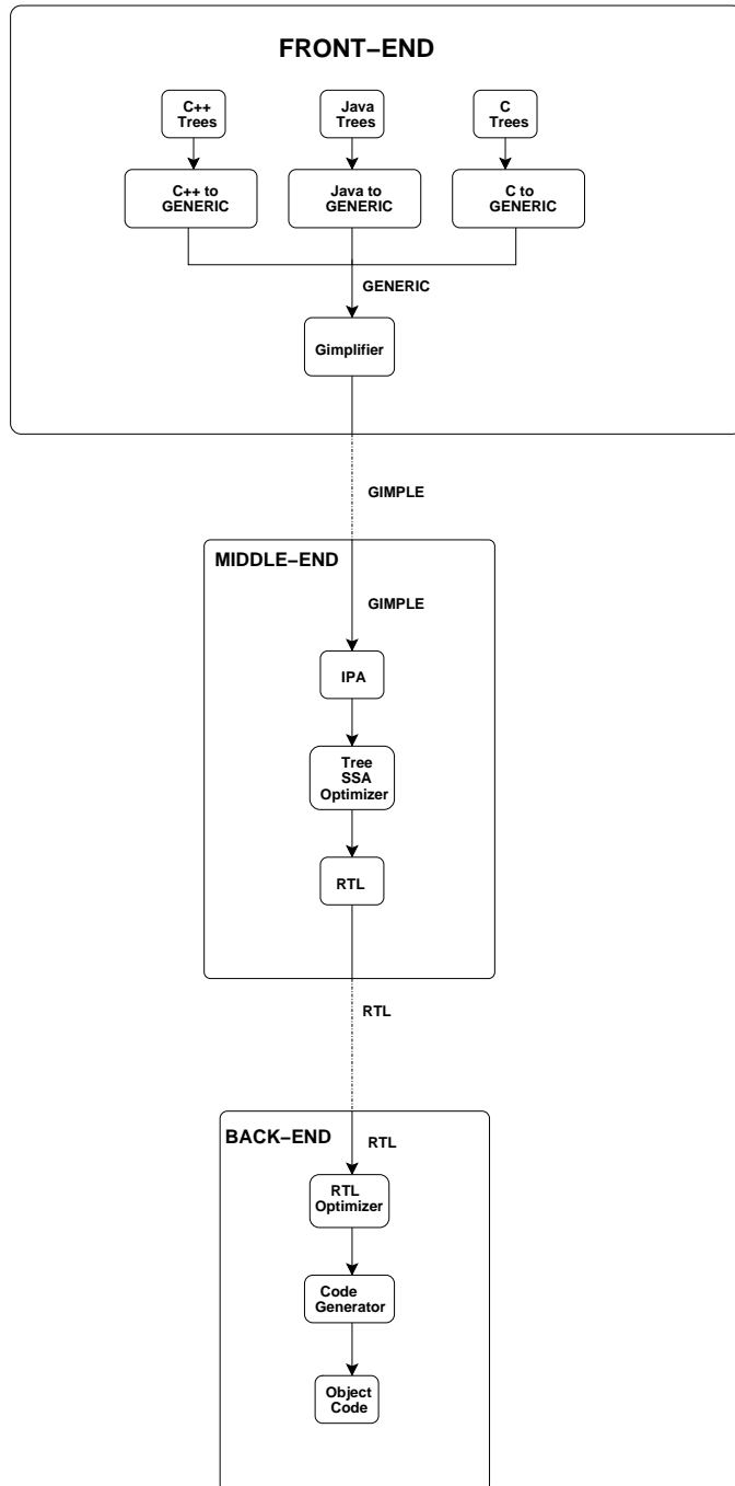
Figure 2: The GCC compilation process adapted from Red Hat Magazine. [35]
