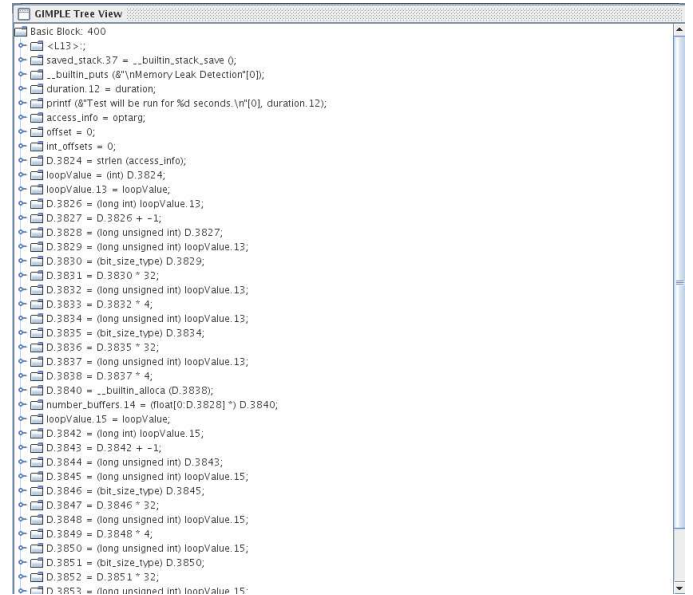
Figure 8: An example basic block with more statements than usual shown in the GIMPLE Tree view of GDE.
