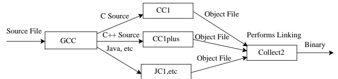
Figure 10: The GCC calling process. Actual file compilation and linking are done by files called by the gcc compiler driver.
