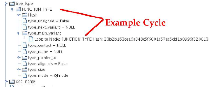
Figure 9: An example cyclic GIMPLE access, the cycle is detected and reported by GDE.
