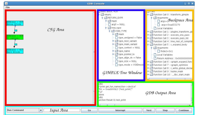
Figure 11: The GDB Console of GDE.
