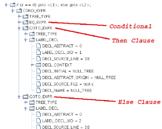
Figure 14: Using GDE to get information about a COND_EXPR .
