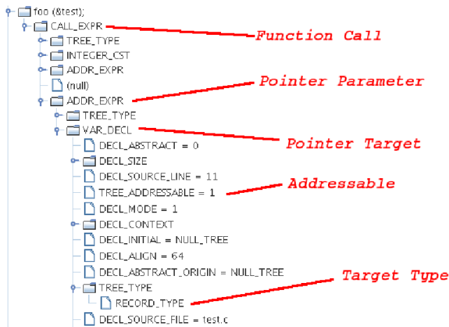
Figure 15: Using GDE to see how a particular statement is gimplified.
