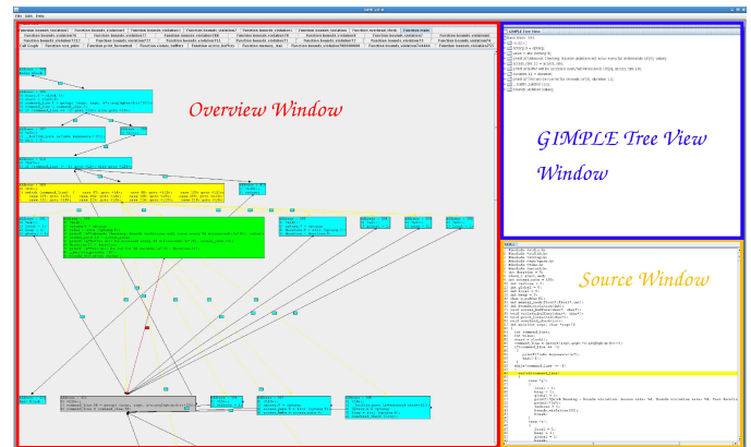
Figure 5: The GDE user interface
