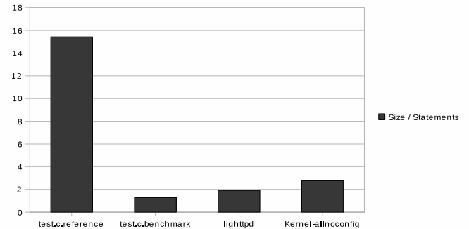
Figure 12: Database size vs. number of statements. Although the ratio is high for test.c.reference , the overall size is 664kB.
