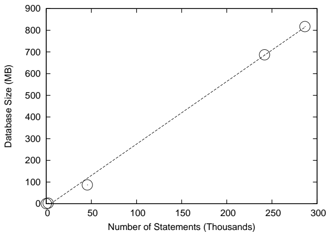
Figure 13: Database size vs.number of statements for each test file.
